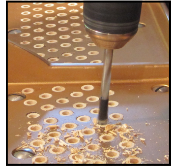
Reaming for tuning pins.
