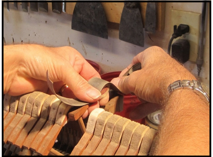
Hammers being filed to remove cut marks.
